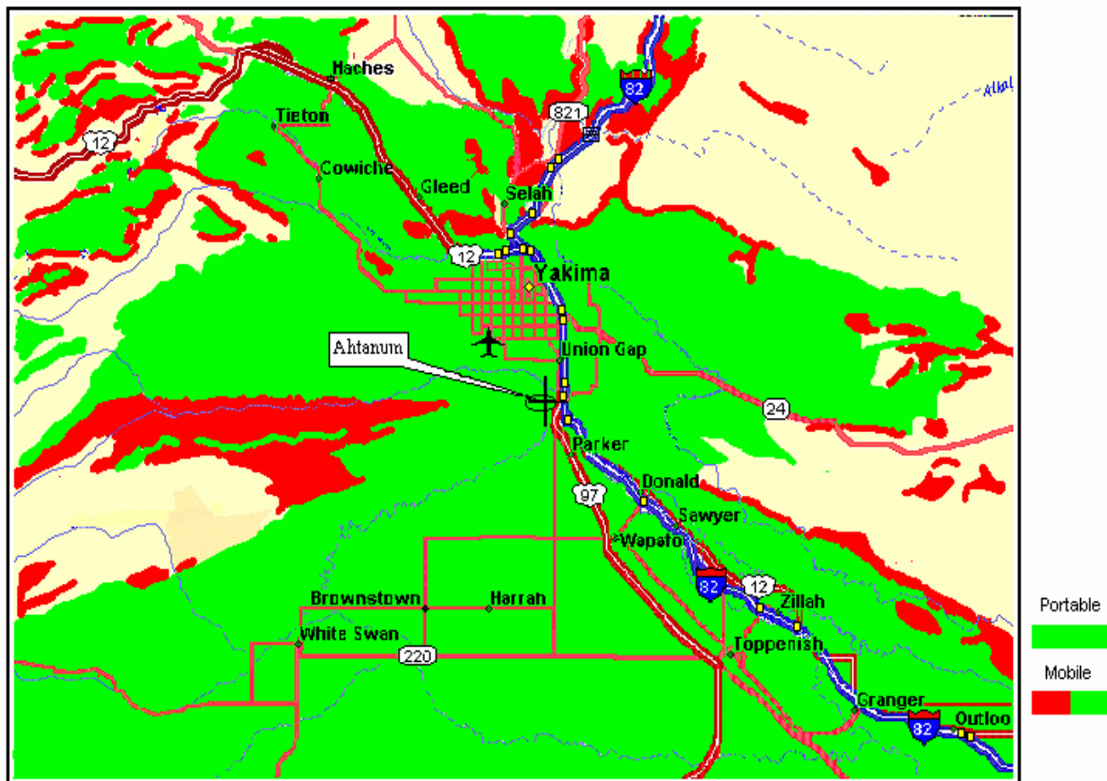
Predicted Area Coverage for Ahtanum UHF System
