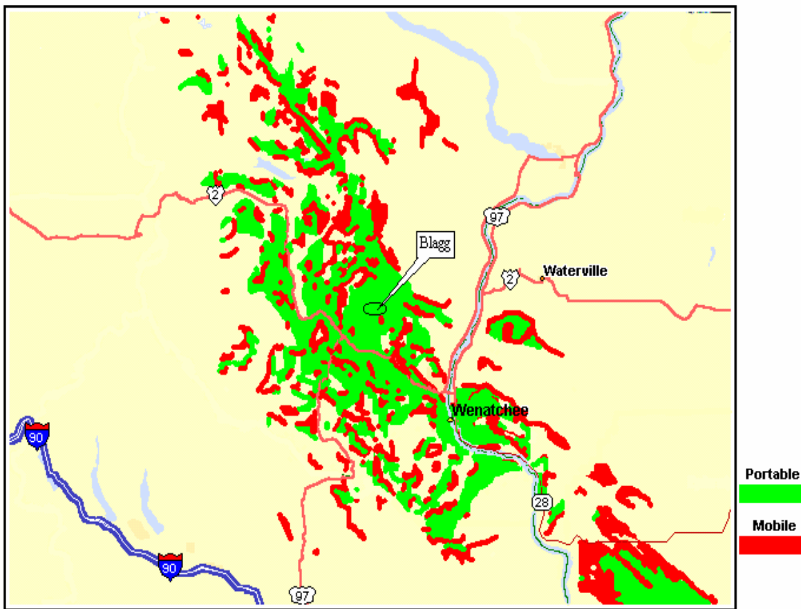
Predicted Area Coverage for Blagg UHF System
