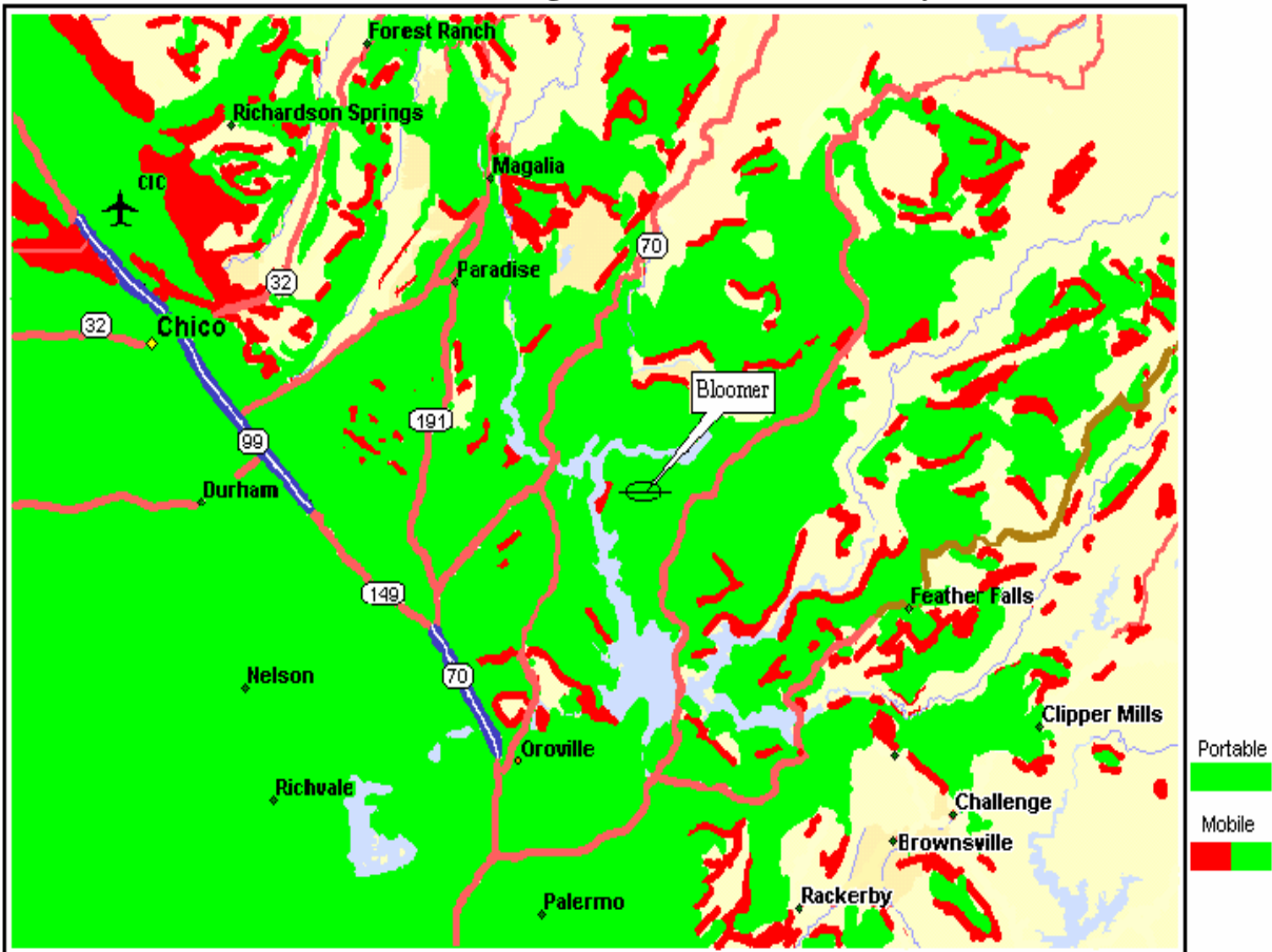
Predicted Area Coverage for Bloomer UHF System
