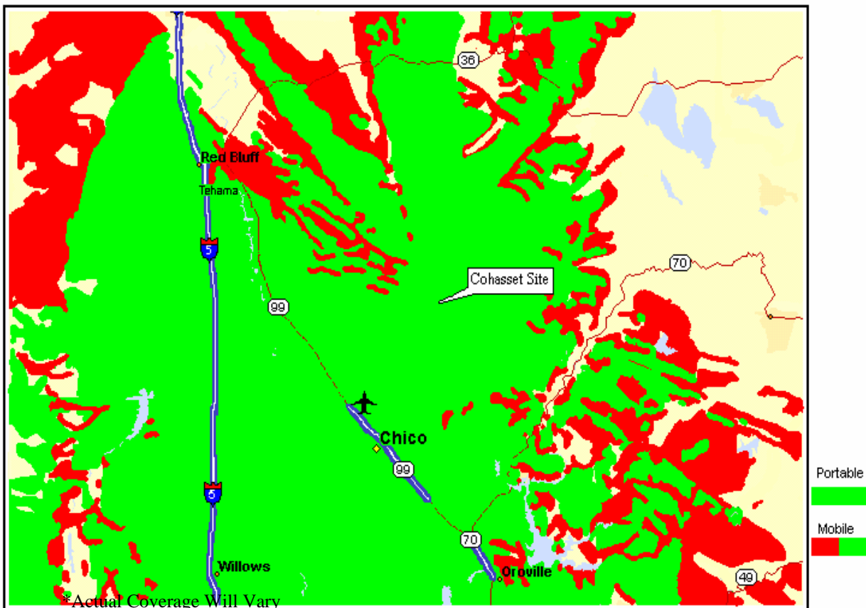
Predicted Area Coverage for Cohasset UHF System
