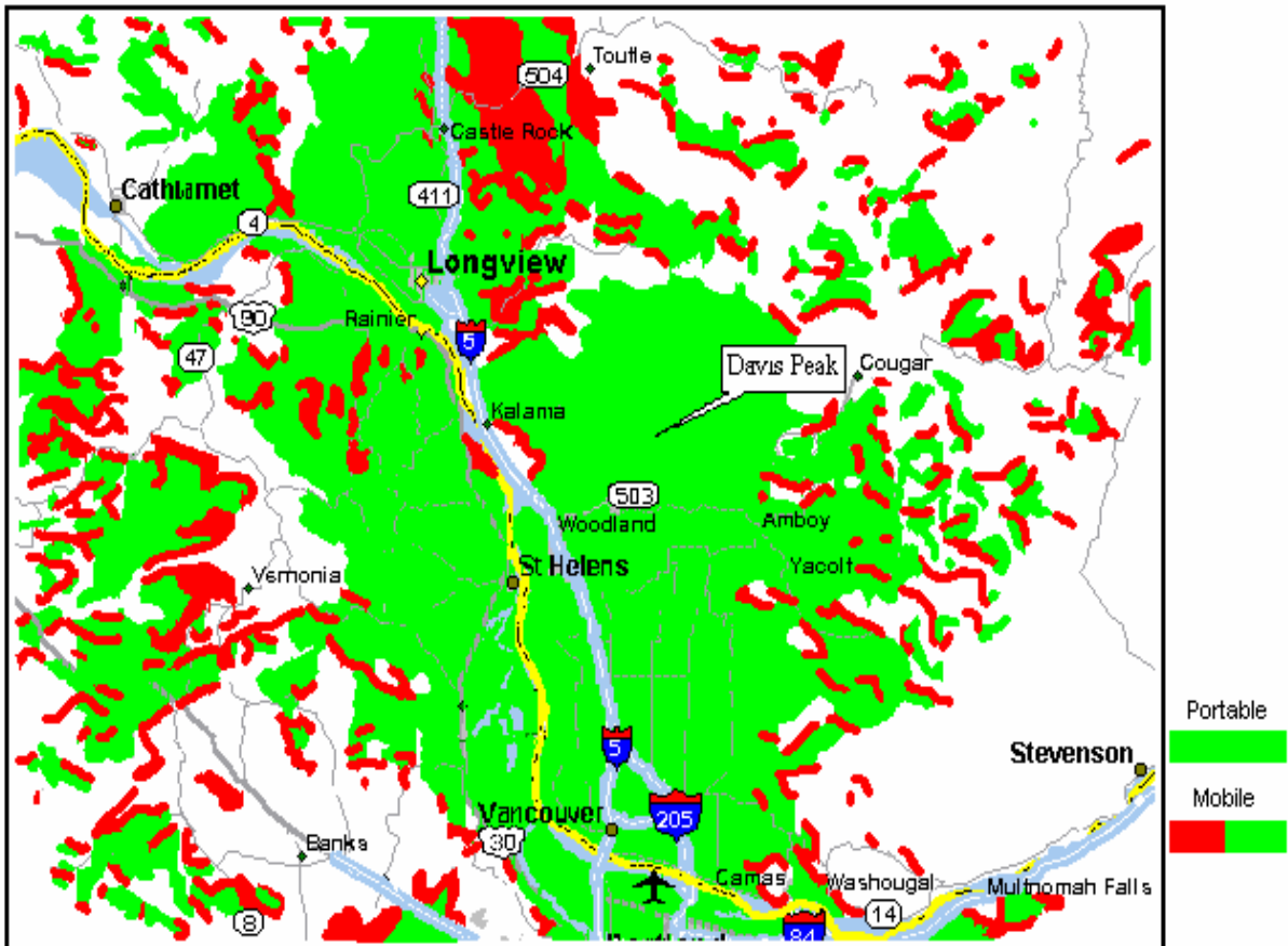
Predicted Area Coverage for Davis Peak UHF System
