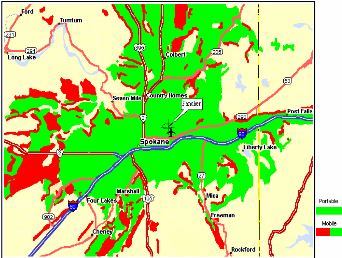
Predicted Area Coverage for Fancher UHF System
