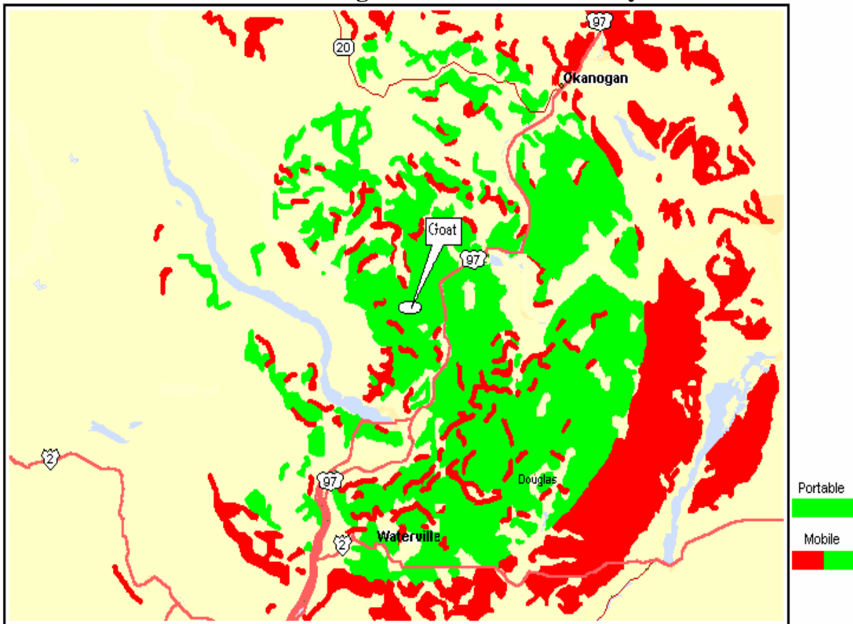
Predicted Area Coverage for Goat Mtn. UHF System
