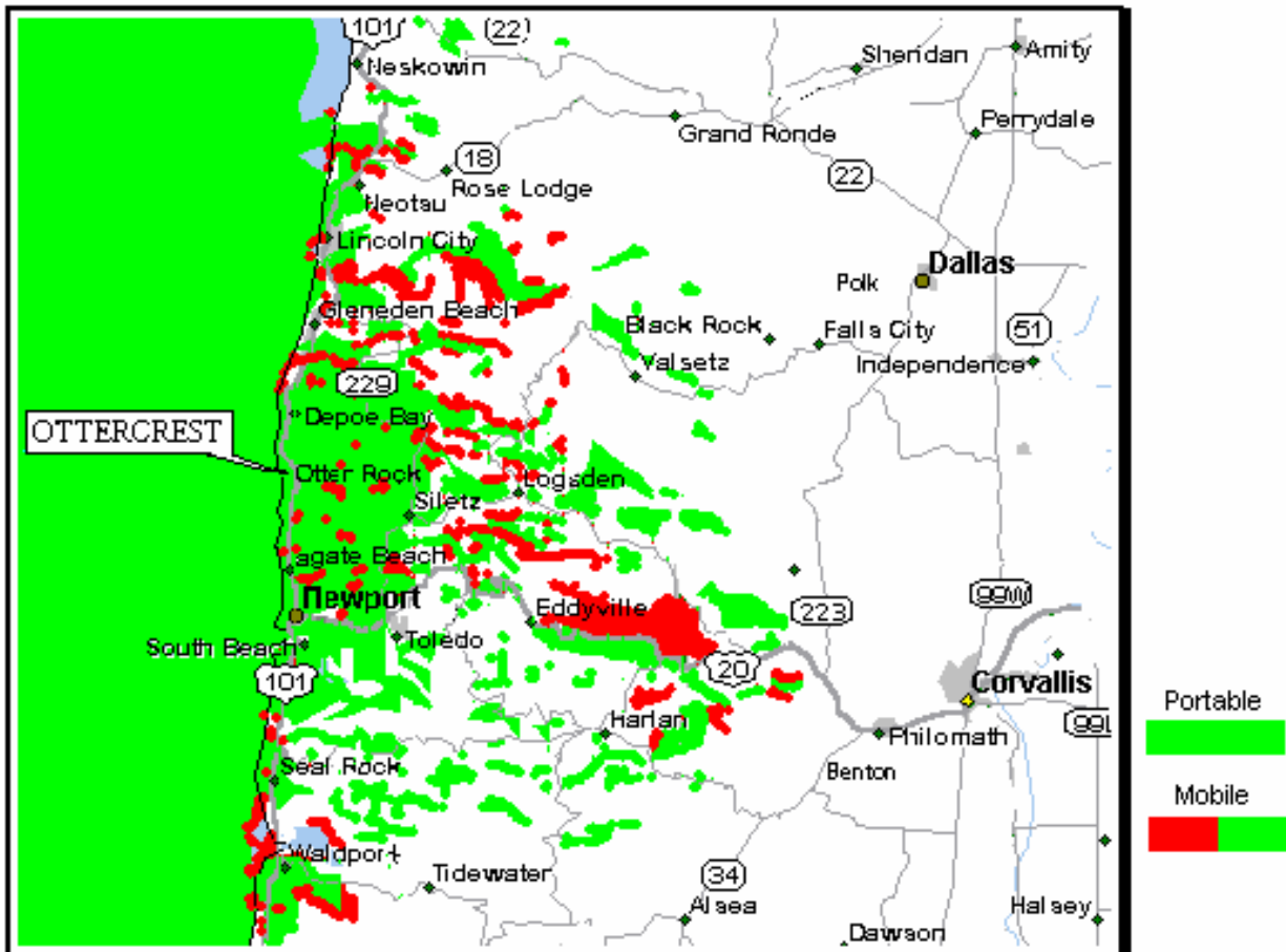
Predicted Area Coverage for Ottercrest UHF System
