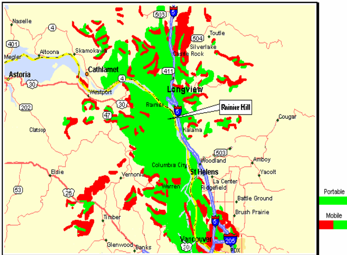
Predicted Area Coverage for Rainier Hill UHF System
