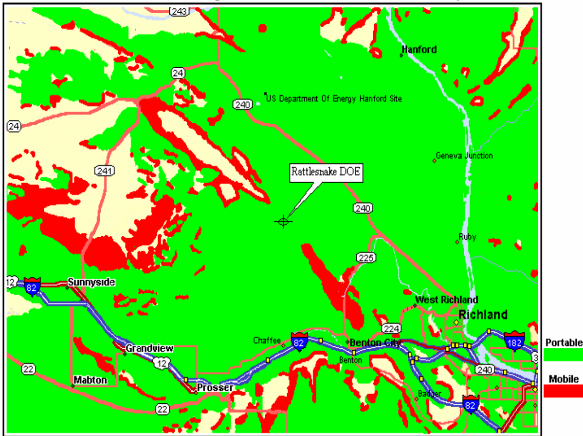
Predicted Area Coverage for Rattlesnake DOE UHF System
