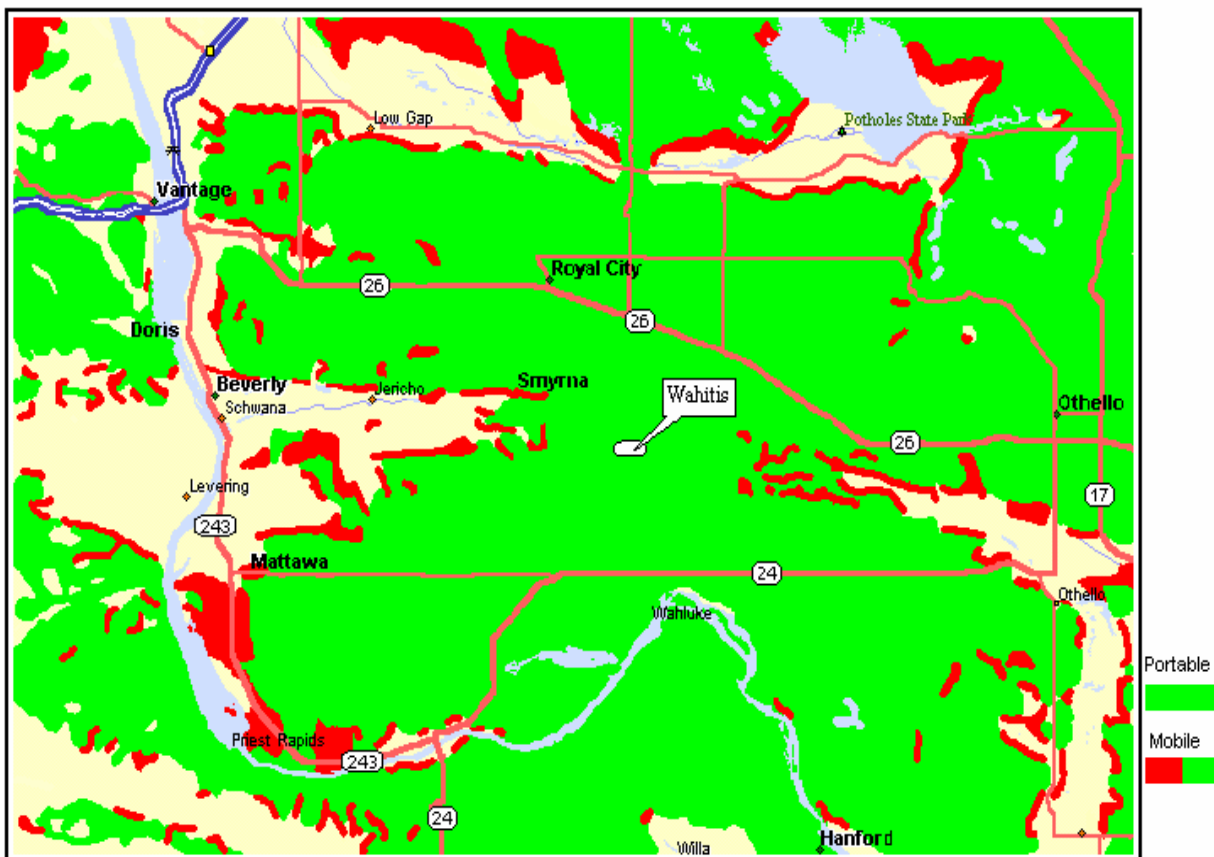
Predicted Area Coverage for Wahitis UHF System
